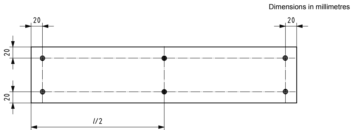
Figure 2 — Measuring points for determination of thickness ( t )
