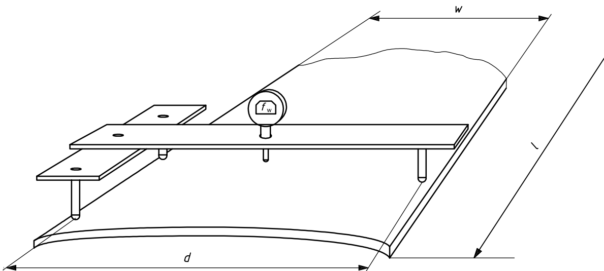
Figure 7 — Determination of width flatness ( f_w )
