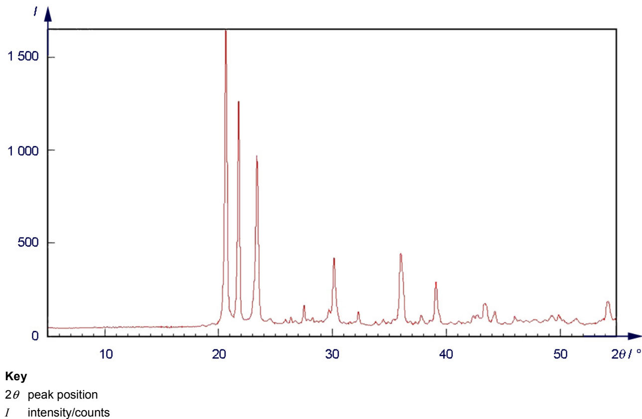
Figure B.2 — An X-ray diffraction scan of crystalline tridymite
