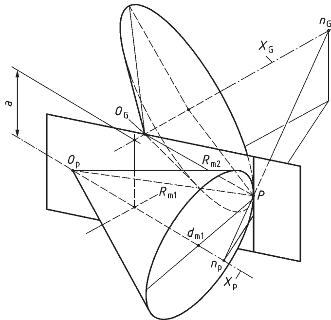
Figure A.2 — Schematic of hypoid gear
