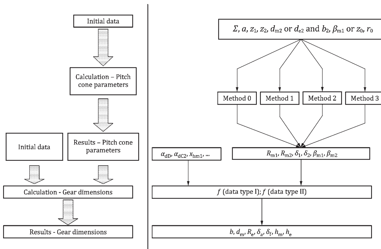
Figure A.1 — Calculation of bevel and hypoid gears
