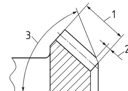
Figure 10 — Bevel gear depthwise tapers
