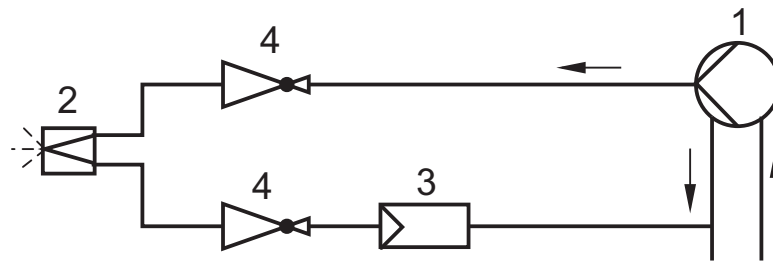
Figure F.3 — Oil burners with spill-back nozzle and without nozzle shut-off valve
