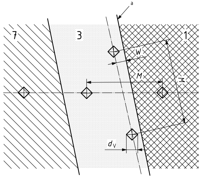
a) Vickers hardness ( d_V/2 \leq W \leq d_V )
