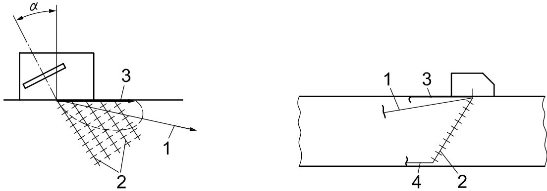
a) Generation of creeping waves
