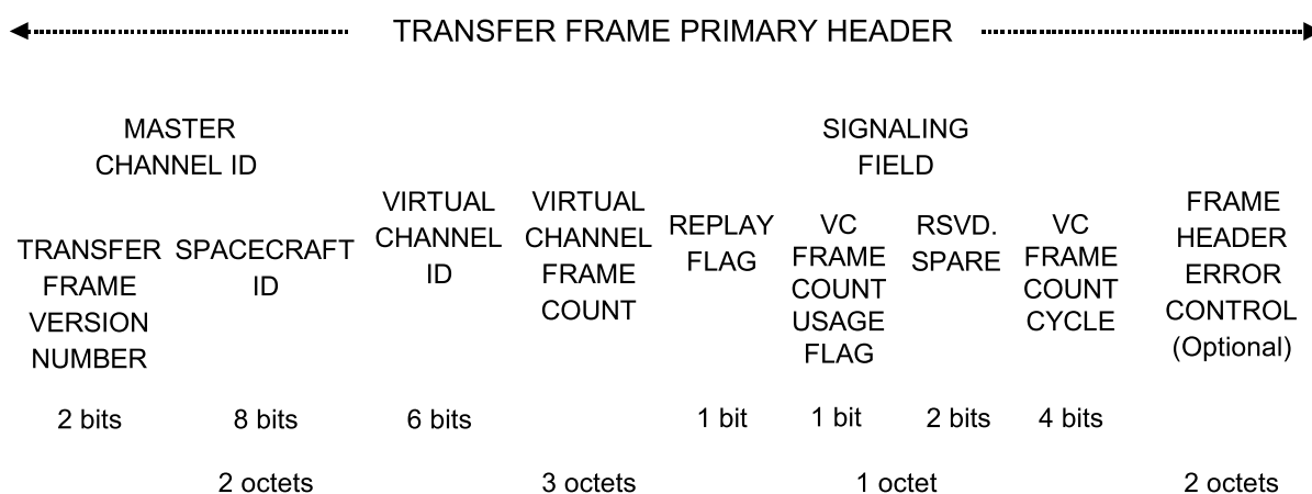
Figure 4-2: Transfer Frame Primary Header
