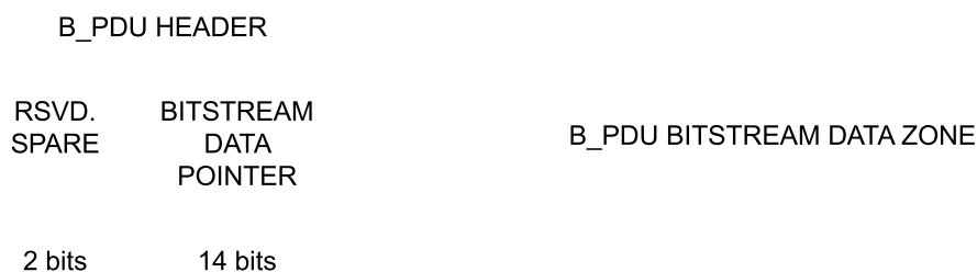
Figure 4-4: Bitstream Protocol Data Unit (B_PDU)
