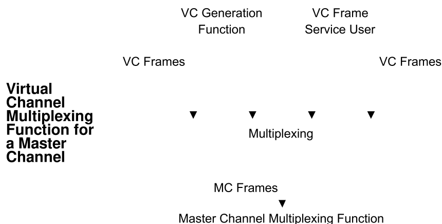
Figure 4-16: Abstract Model of Virtual Channel Multiplexing Function
