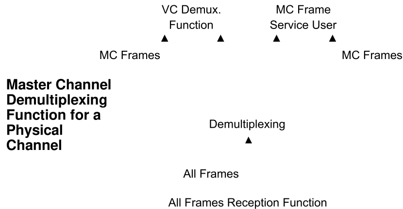
Figure 4-26: Abstract Model of Master Channel Demultiplexing Function
