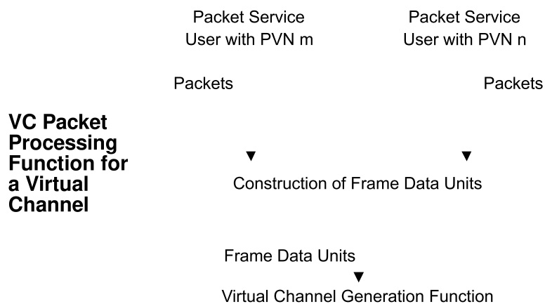
Figure 4-13: Abstract Model of VC Packet Processing Function
