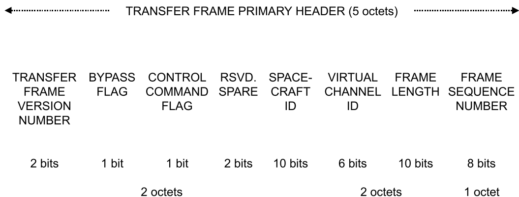
Figure 4-2: Transfer Frame Primary Header
