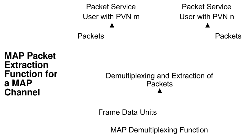
Figure 4-20: Abstract Model of MAP Packet Extraction Function
