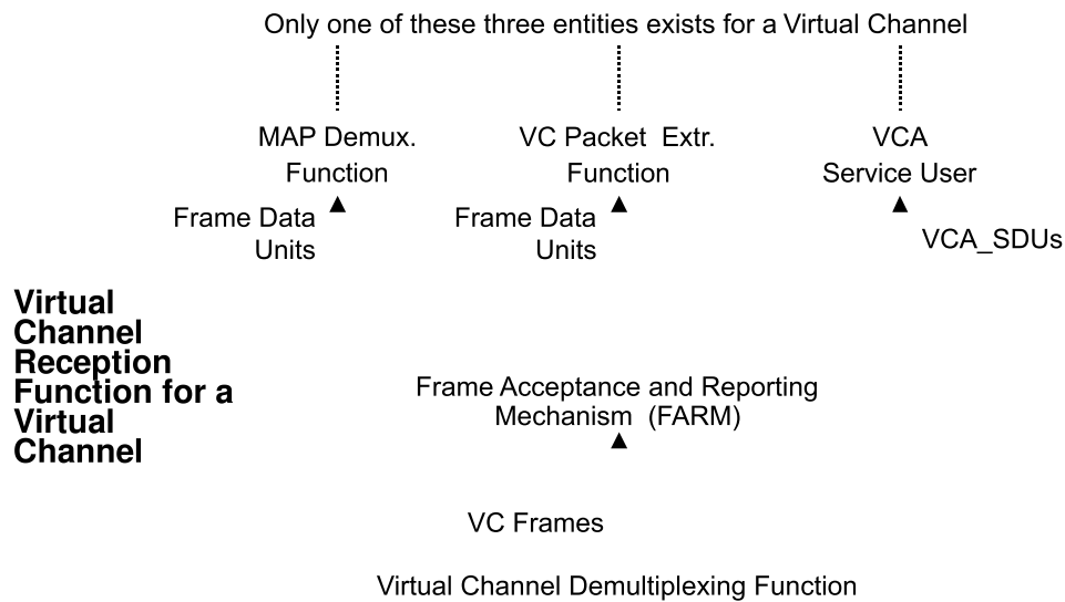
Figure 4-24: Abstract Model of Virtual Channel Reception Function
