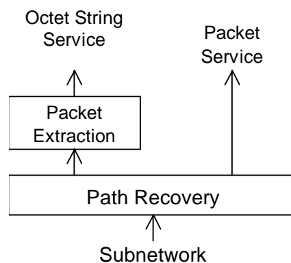
Figure 4-6: Internal Organization of Protocol Entity (Receiving End)
