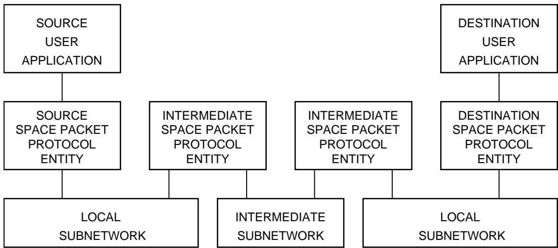
Figure 2-2: Example of a Logical Data Path
