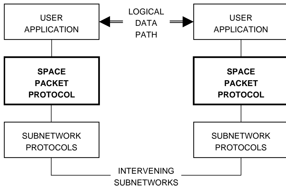
Figure 2-1: Protocol Configuration
