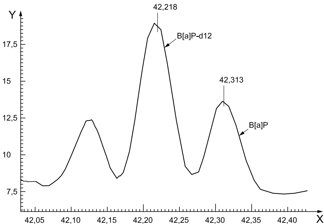
Figure A.1 — Example of a chromatogram of a cigarette smoke extract
