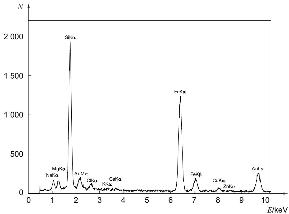
Figure F.2 — Energy dispersive X-ray spectrum obtained from SRM 1866 amosite. The gold peaks originate from the gold specimen grid
