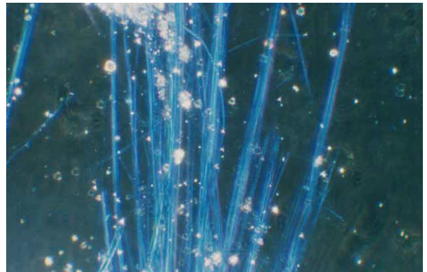
Figure D.16 — SRM 1866 crocidolite in 1,700 RI liquid — Dispersion staining — Fibre lengths normal to polarizer vibration direction
