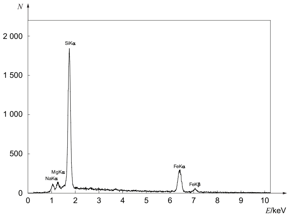
Figure E.2 — Energy dispersive X-ray spectrum obtained from SRM 1866 amosite
