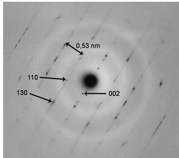
Figure F.12 — Chrysotile SAED pattern
