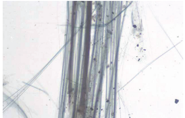
Figure D.14 — SRM 1866 crocidolite in 1,700 RI liquid in plane polarized light — Fibres normal to polarizer vibration direction
