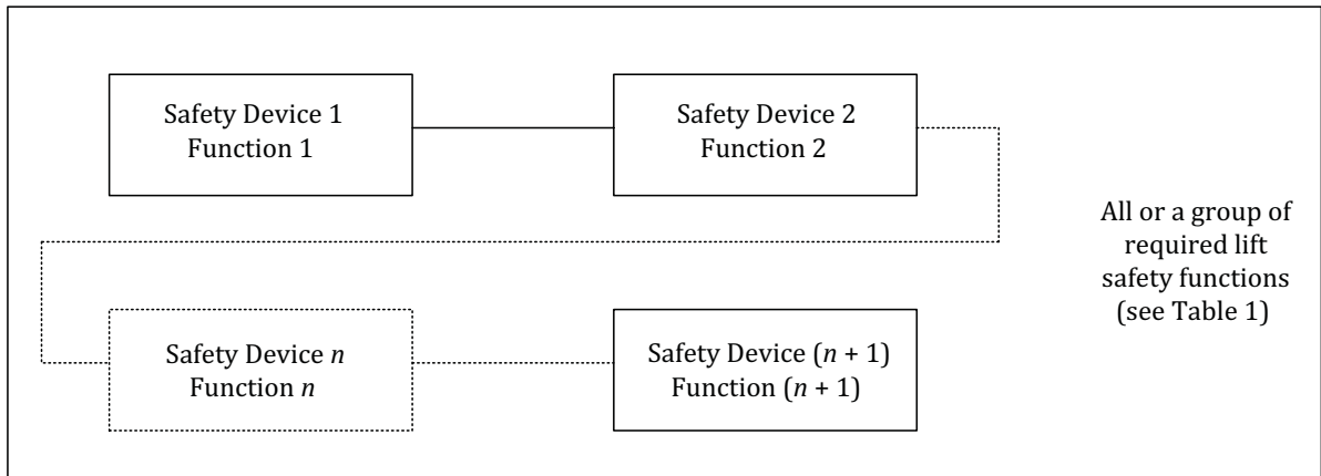
Figure 2 — Safety chain
