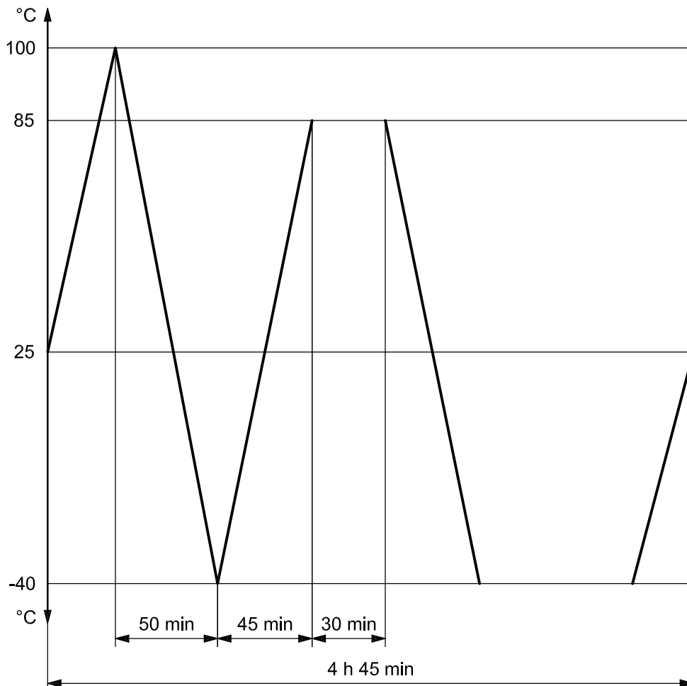
Figure 1 — WFC thermal cycle test
