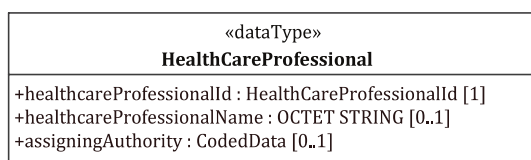
Figure 23 — Structure of HealthCareProfessional
