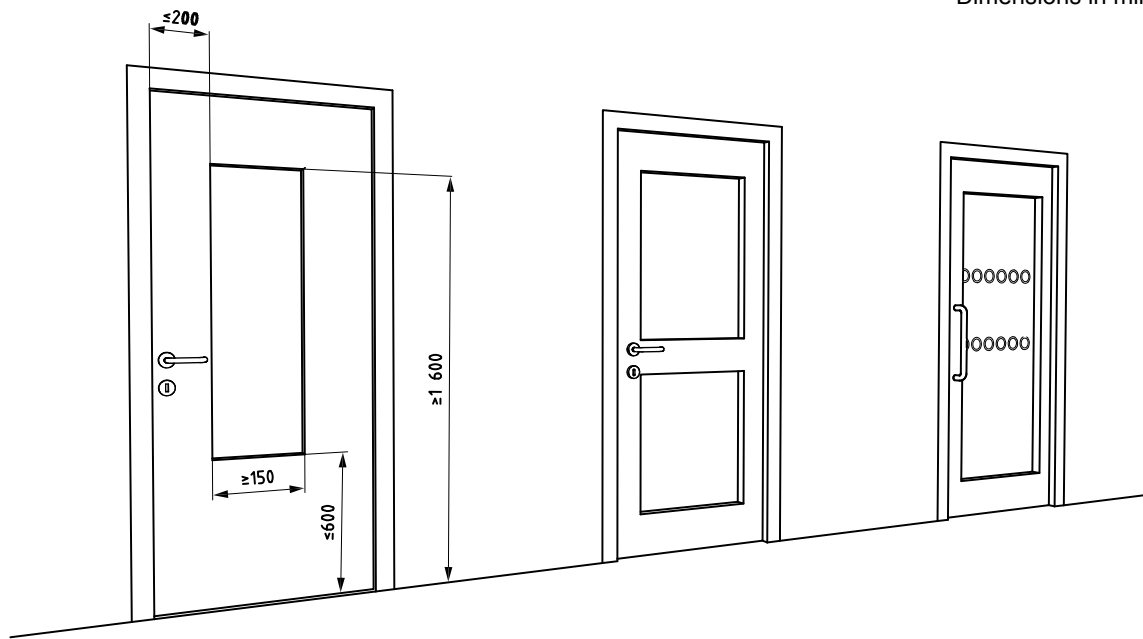
Figure 28 — Examples of doors with glazed viewing panels
