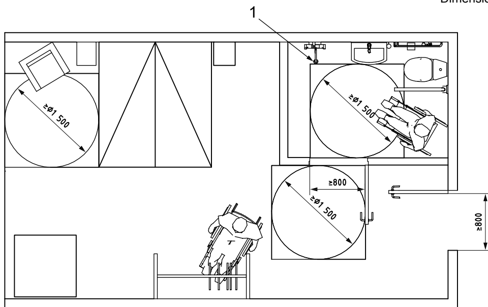
Figure 50 — Example of space allowances for accessible bedroom
