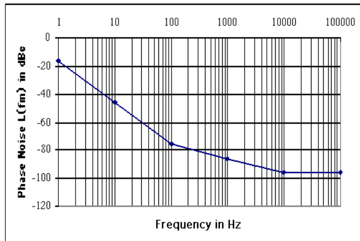
Figure 3-1: Oscillator Phase Noise
