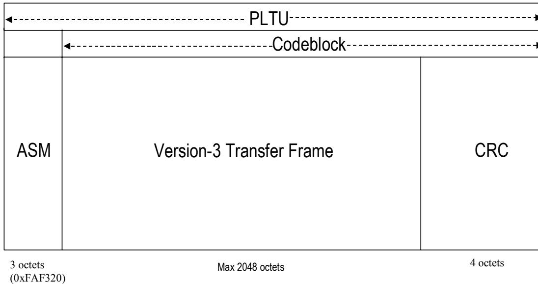
Figure 3-1: Proximity-1 Link Transmission Unit (PLTU)
