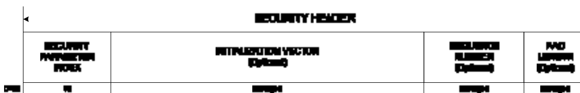
Figure 4-1: Security Header
