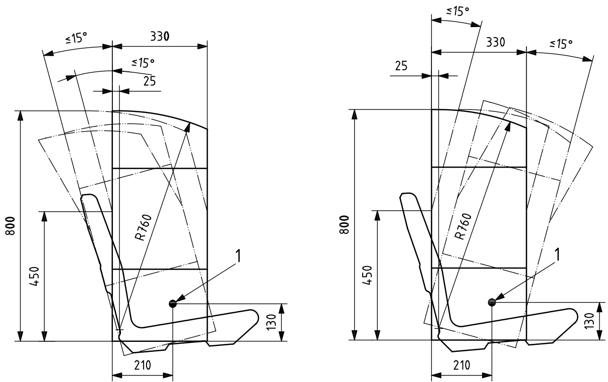
a) DLV side view in vertical and rearward positions
