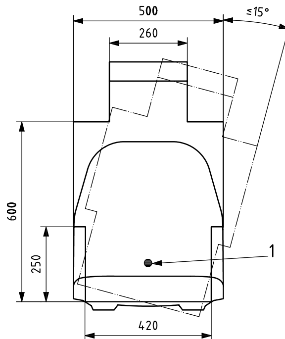
c) DLV front view in leftmost position (may also rotate similarly to the right)
