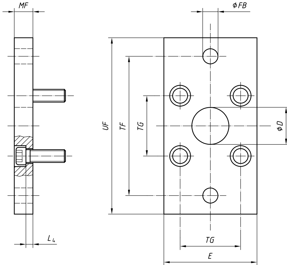
Figure 4 — Head, rectangular flange (MF1) and cap, rectangular flange (MF2)
