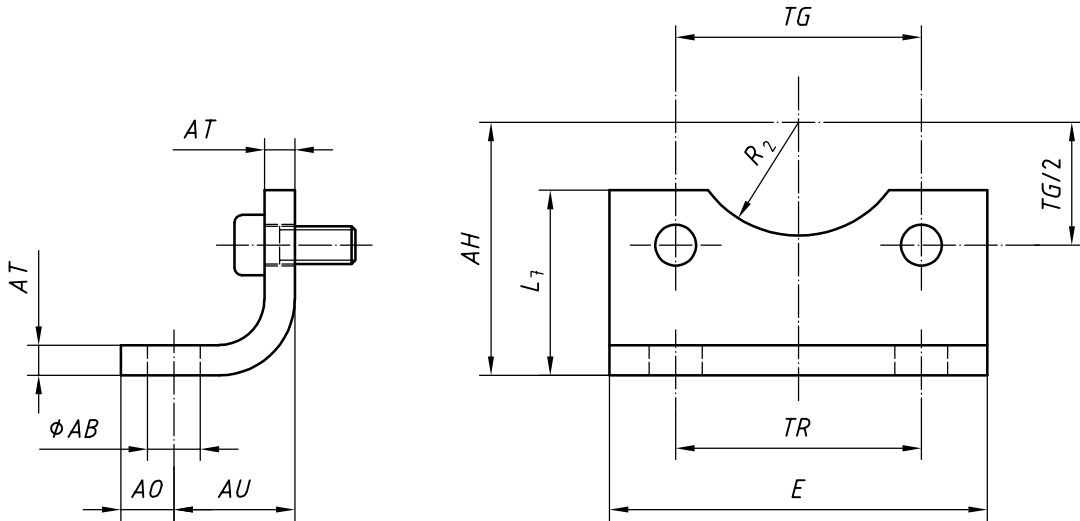
Figure 5 — End angles (MS1)
