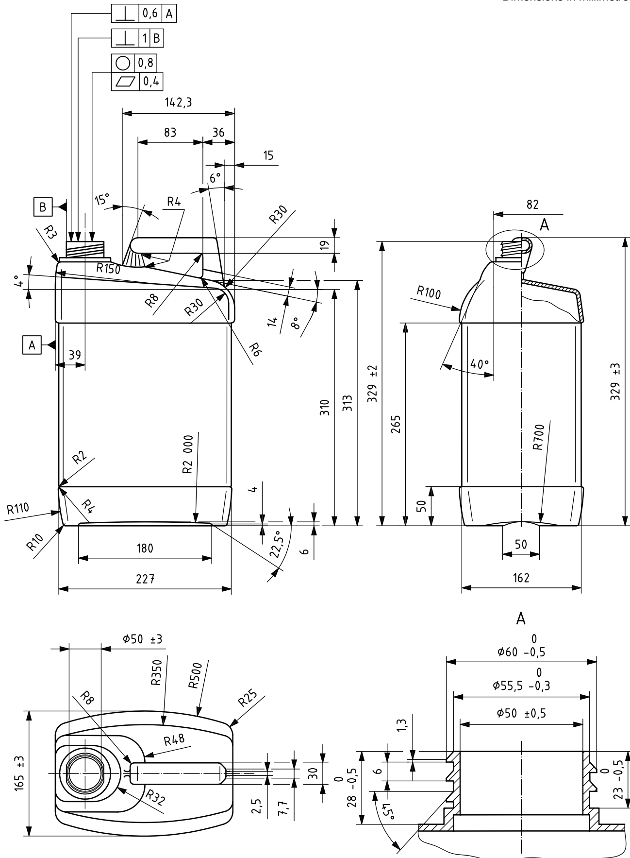
Figure 3 — Reference can
