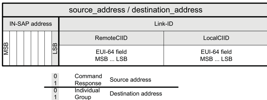
Figure 9 — IN-SAP Source and Destination Address Format
