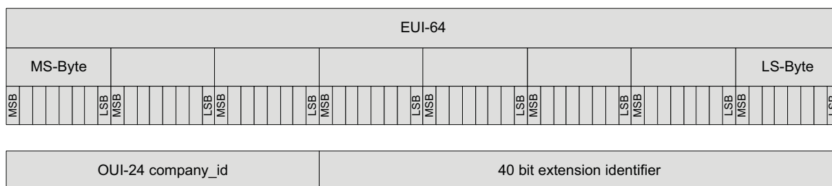
Figure C.1 — EUI-64 format
