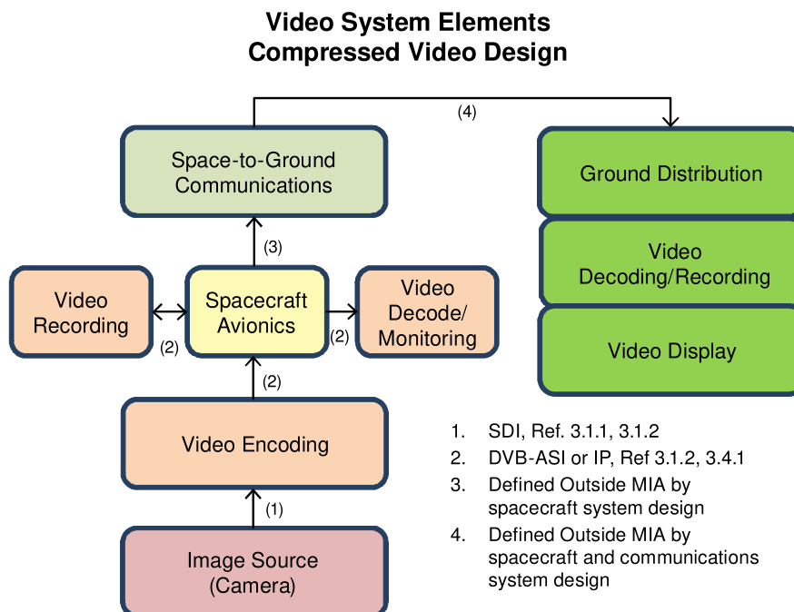
Figure 3-2: Video System Elements—Compressed Video Design
