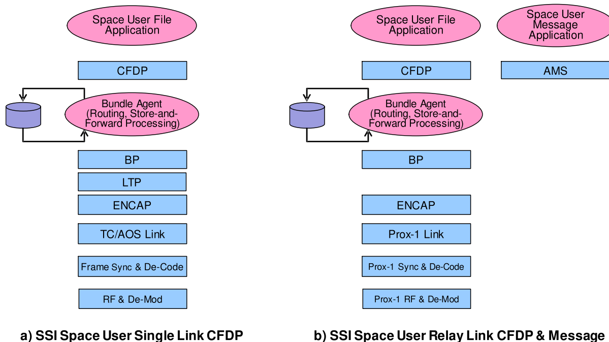
Figure 6-27: SSI Space User DTN Forward-File Building Blocks
