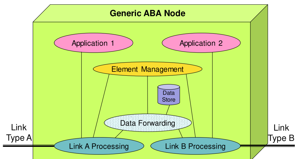
Figure 5-1: ABA Node—Generic Building Block
