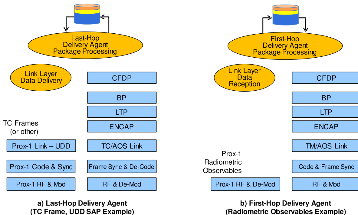
Figure 6-31: SSI Last-Hop/First-Hop Delivery Agent Building Blocks
