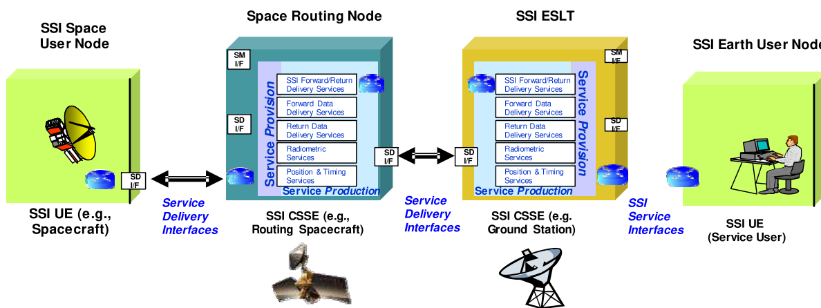
Figure 4-2: SSI End-to-End Run-Time Service Interfaces
