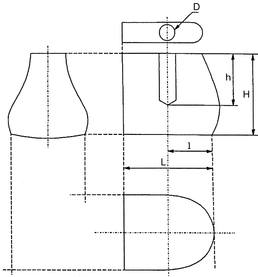
Figure 1 - Test punch for compression energy test
