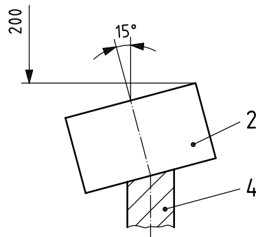
b) Degree of protection against water 2
