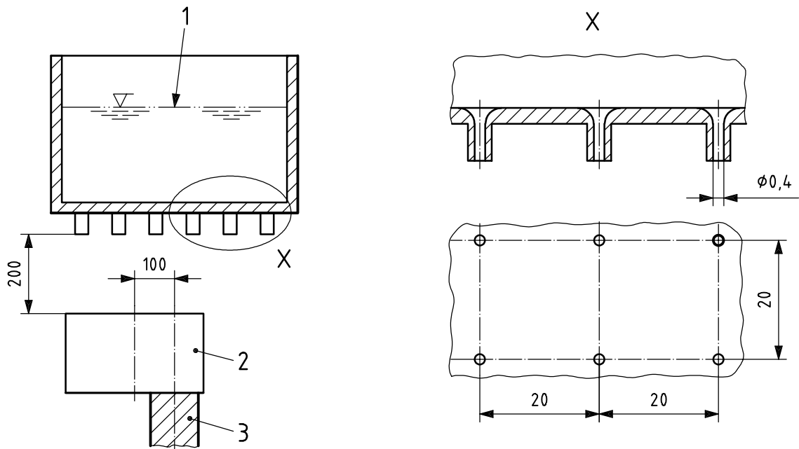
a) Degree of protection against water 1
