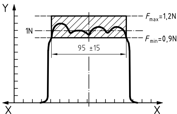
Figure 8 — Distribution of impact force for determining the protection against high-pressure/steam-jet cleaning, degree of protection against water 9K
