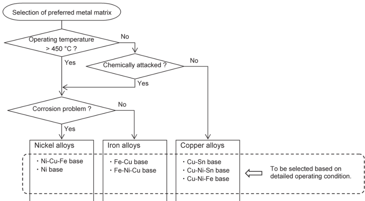
Figure A.1 — Selection procedure of a bearing metal matrix for bearings containing dispersed solid lubricants
