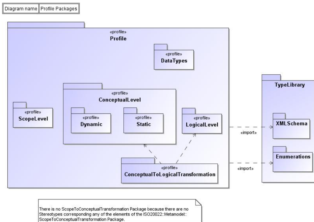
Figure A.1 — Example of Profile Packages
