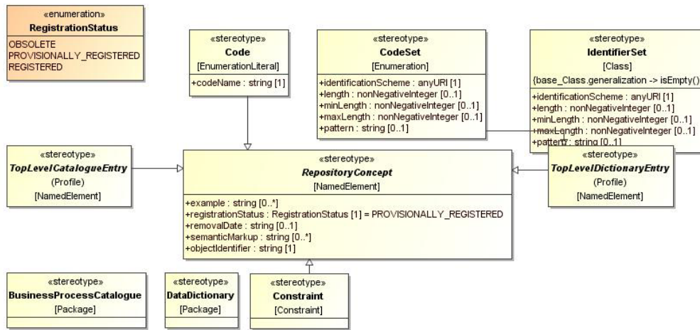
Figure A.2 — Example of ISO20022 Level Stereotypes
