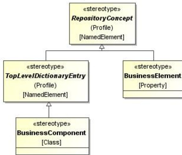
Figure A.4 — Example of Conceptual Static Stereotypes
