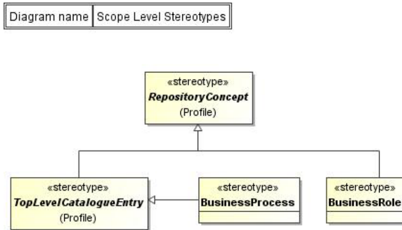
Figure A.8 — Example of Scope Level Stereotypes
