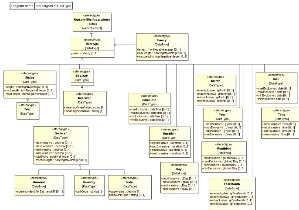
Figure A.6 — Example of stereotypes of DataType
