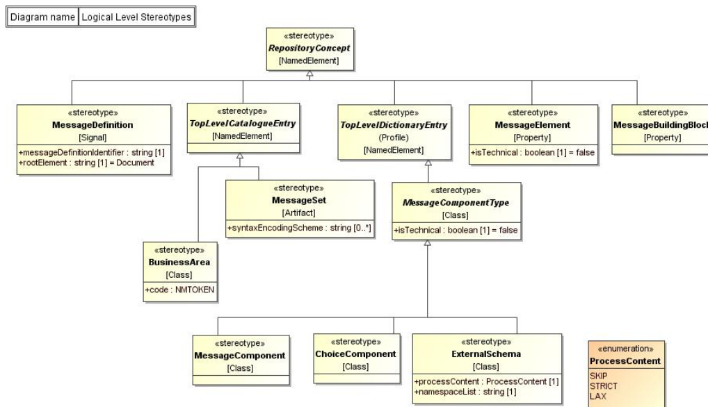
Figure A.7 — Example of Logical Level Stereotypes
