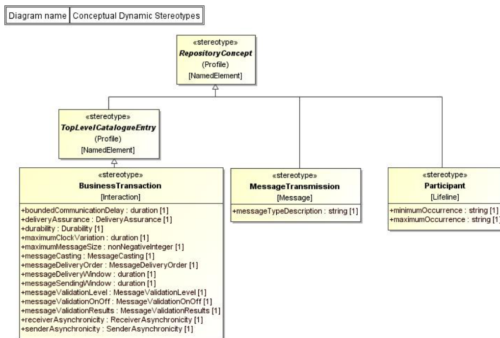
Figure A.3 — Example of conceptual Dynamic Stereotypes
