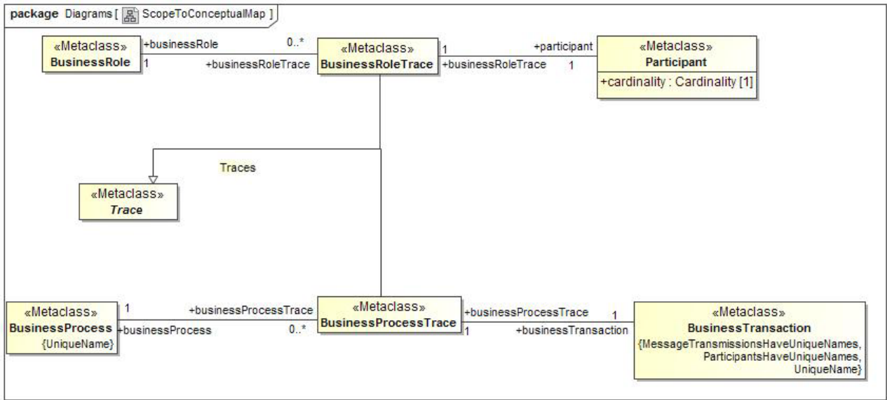
Figure 10 — Scope to Conceptual level mapping
