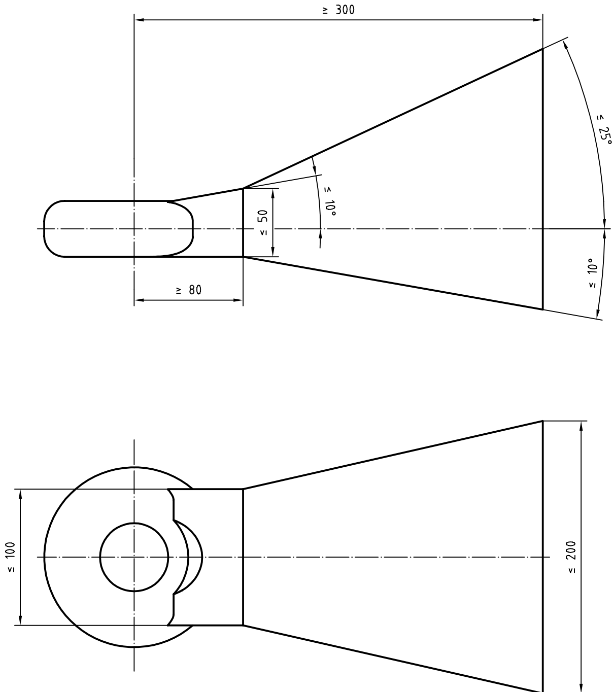
Figure 3 — Hitch shank dimensions
