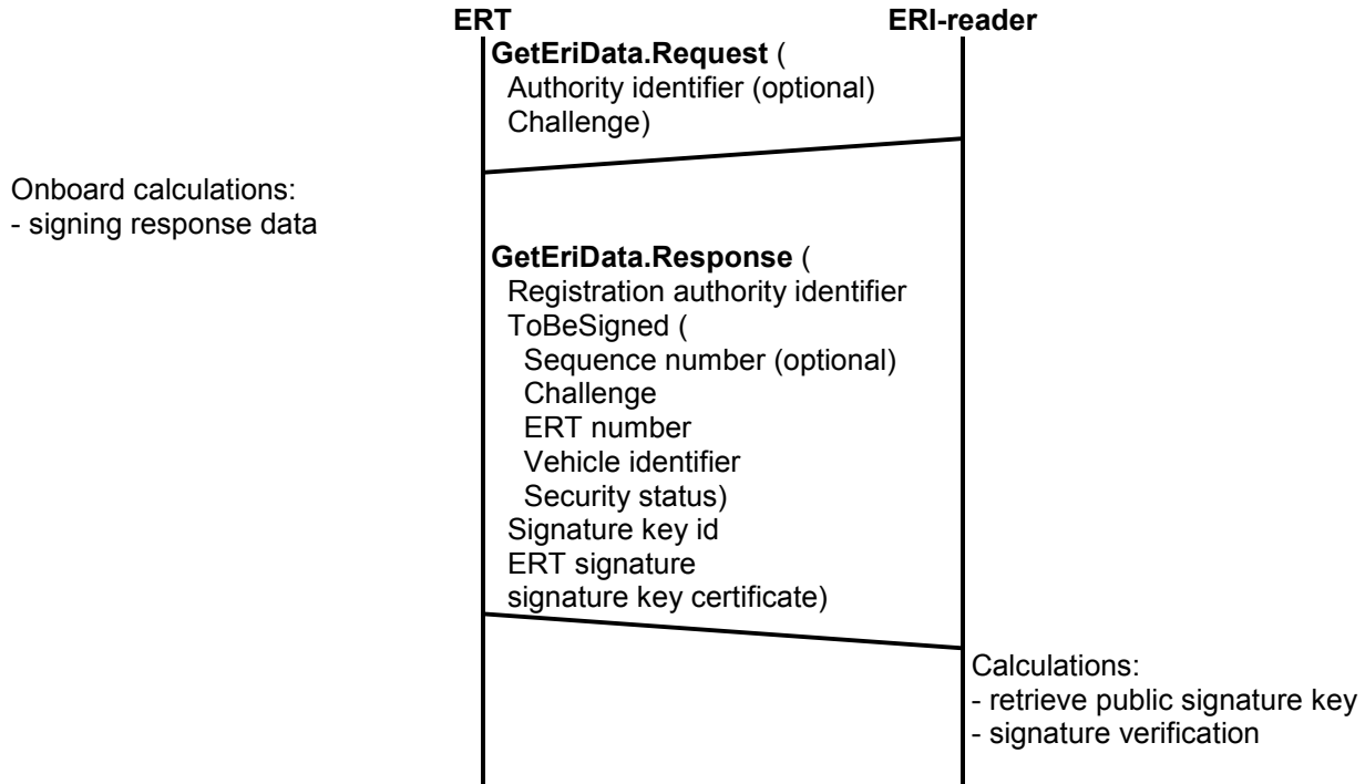
Figure B.4 — ERI from ERT that only supports authentication
