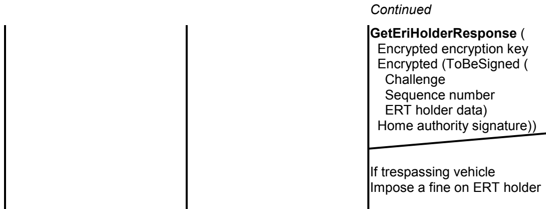
Figure B.7 — Enforcement of HOV or HGV lane infringement
