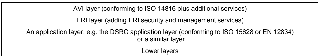
Figure 9 — Protocol stack for the short-range air interface
