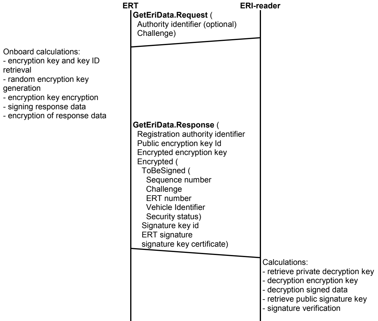
Figure B.3 — ERI from an ERT that supports both confidentiality and authentication
