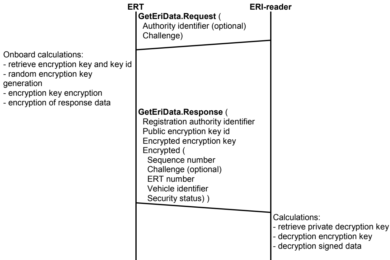
Figure B.5 — ERI from ERT that only supports confidentiality
