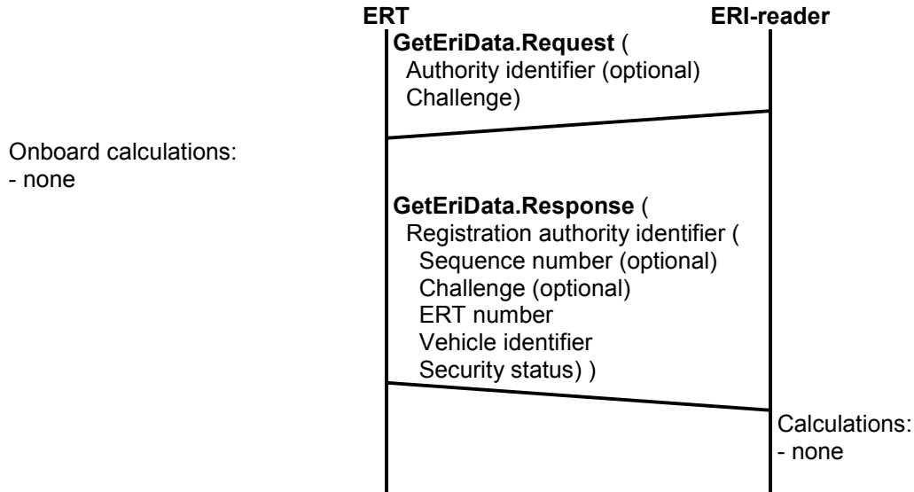
Figure B.6 — ERI from ERT with no security services
