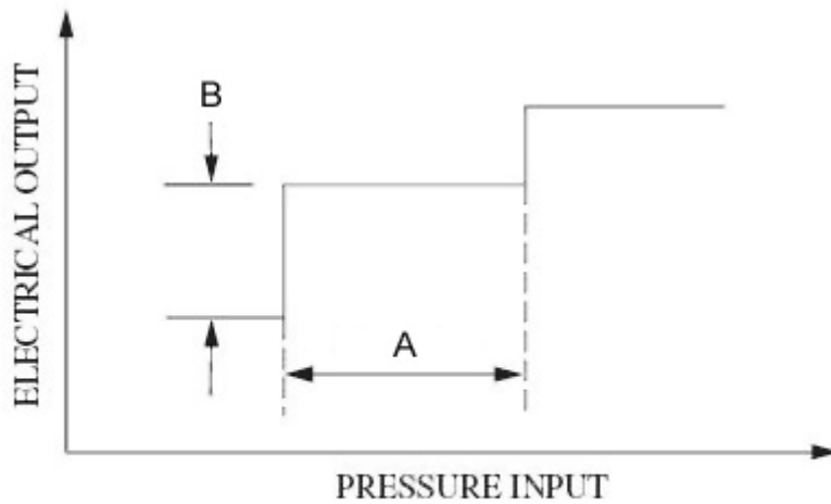
Figure A.18 — Illustration of hysteresis (from Freeman and others [8], Figure 28)
