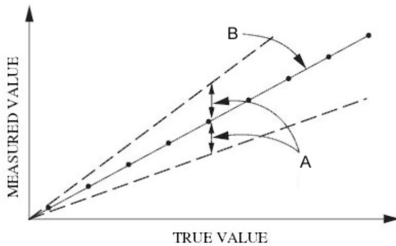
Figure A.14 — Illustration of zero error (from Freeman and others [8], Figure 24)
