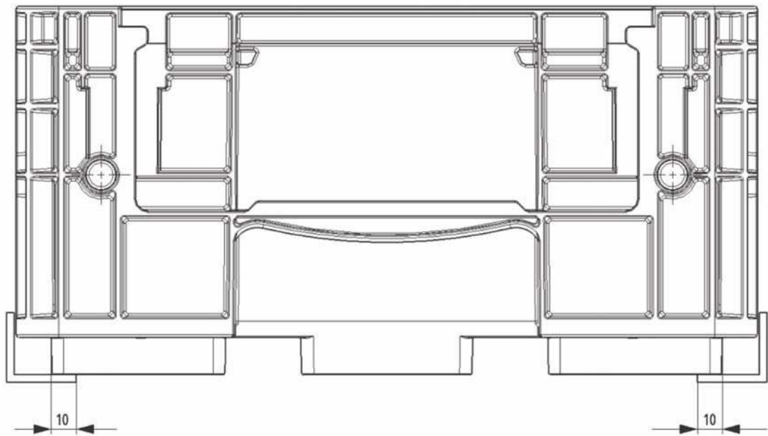
Figure A.3 — Positioning of container during testing
