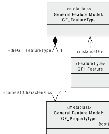
Figure C.1 — Feature Instance model
