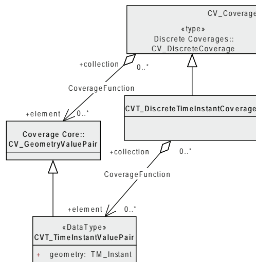
Figure C.2 — Specialized coverage type for time-series
