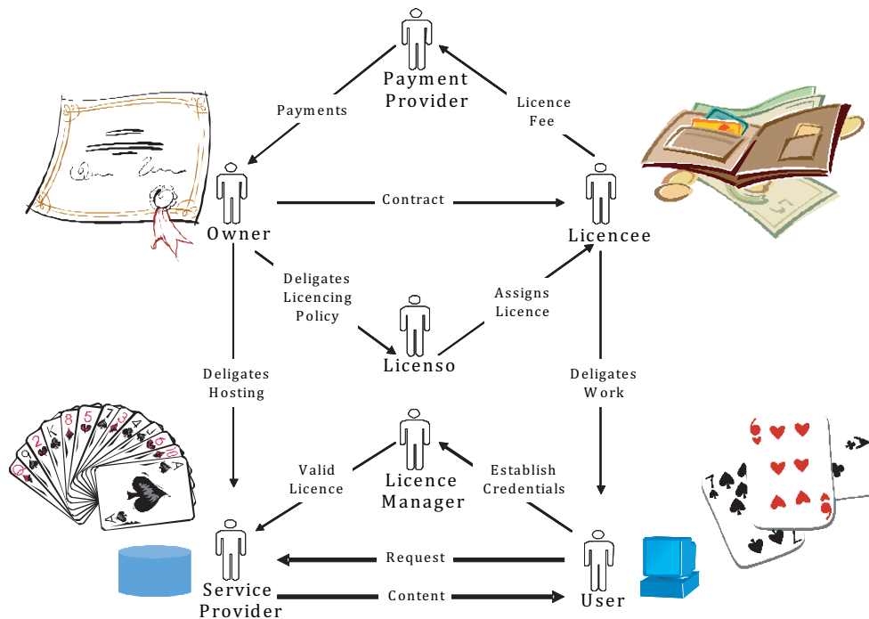
Figure C.1 — GeoDRM game — Interactive role playing
