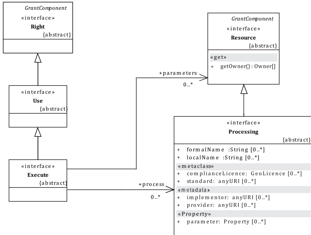
Figure B.7 — Processing right
