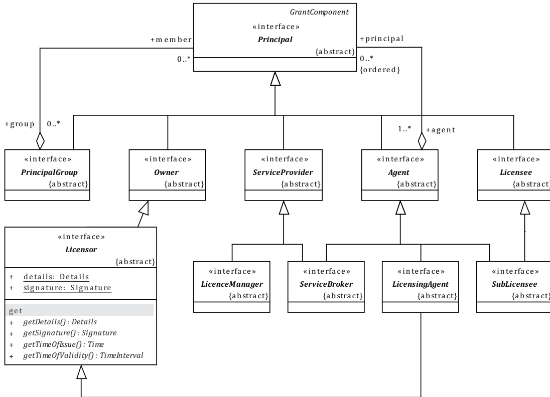
Figure 13 — Various principals in a GeoDRM system
