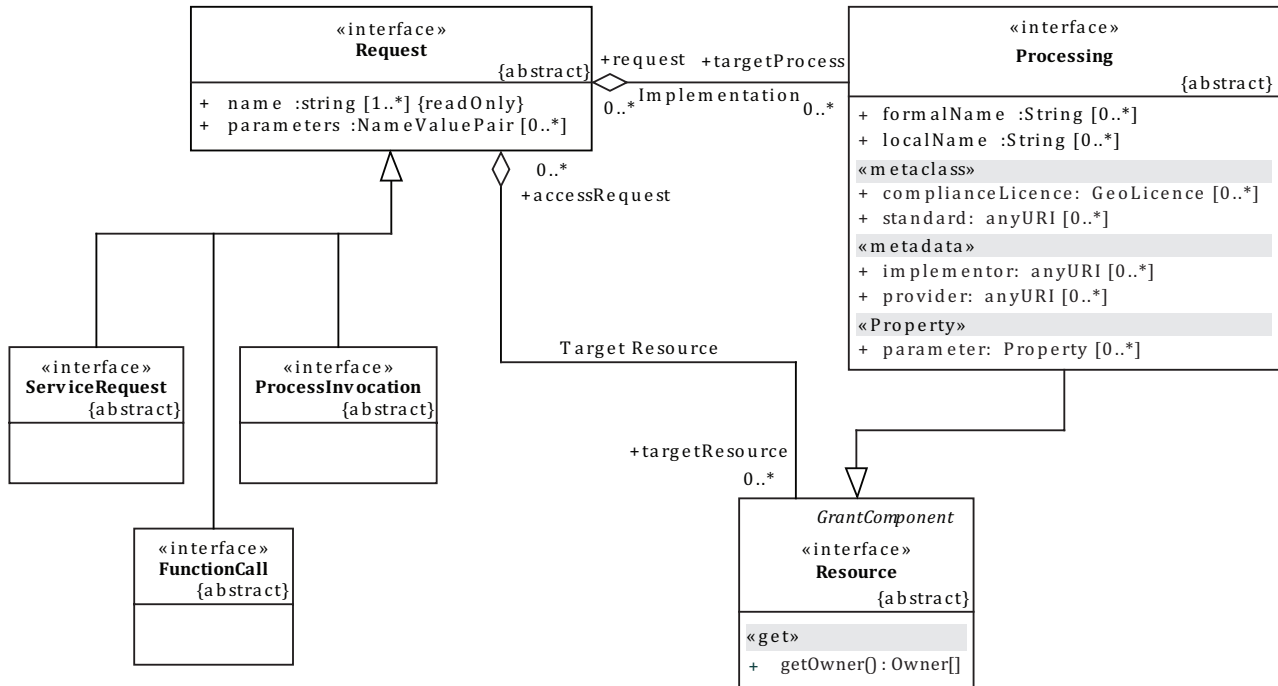
Figure B.9 — Request
