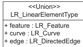
Figure 17 — Context diagram: LR_LinearElementType
