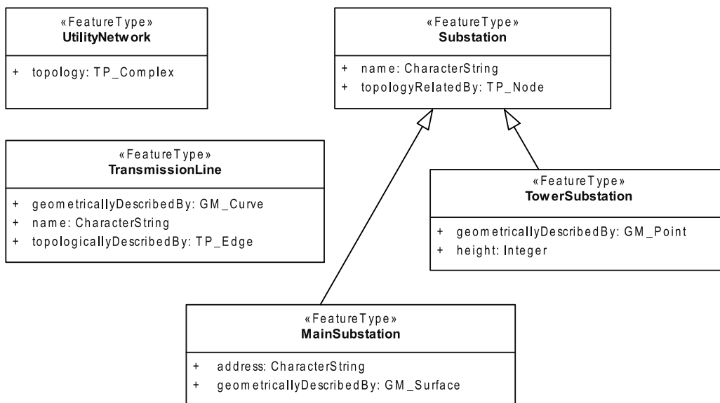
Figure C.2 — Example of application schema for utility network
