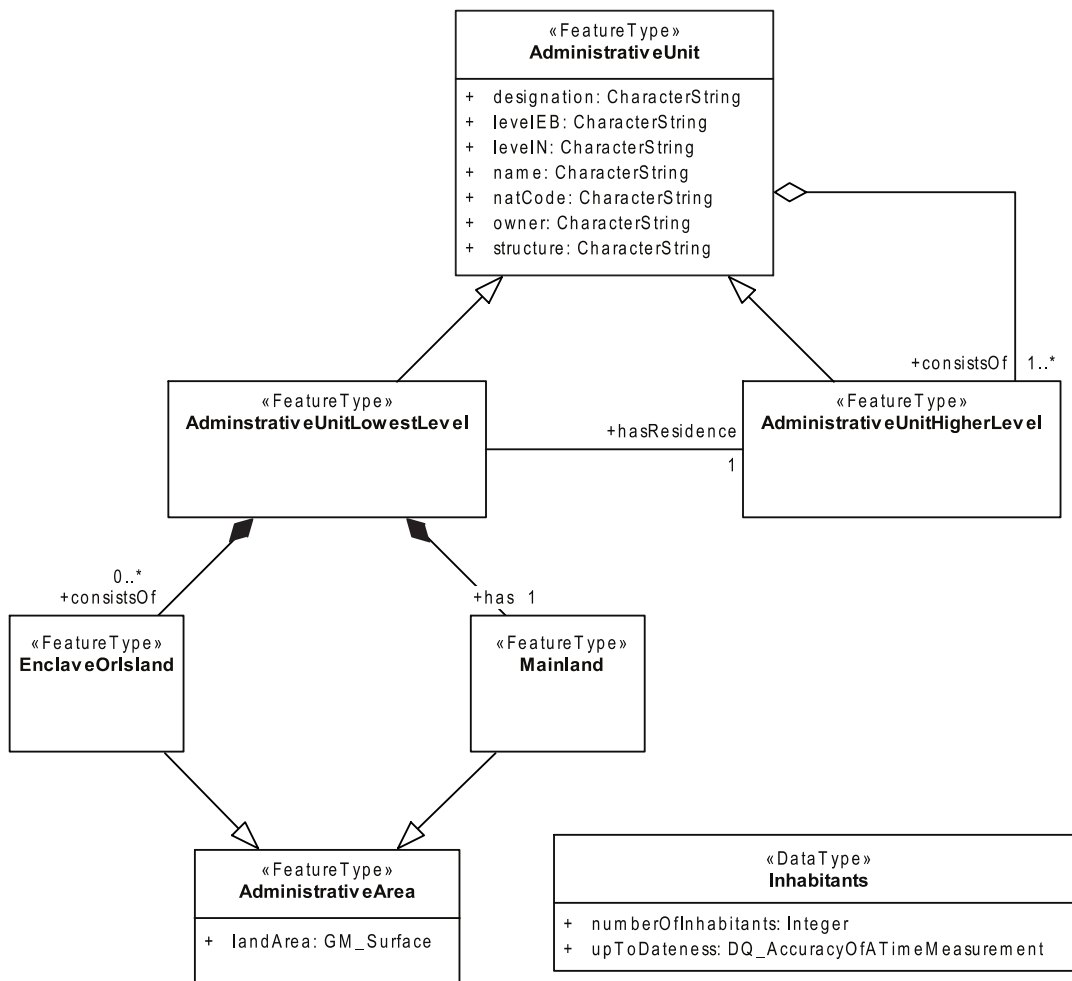
Figure C.3 — UML application schema
