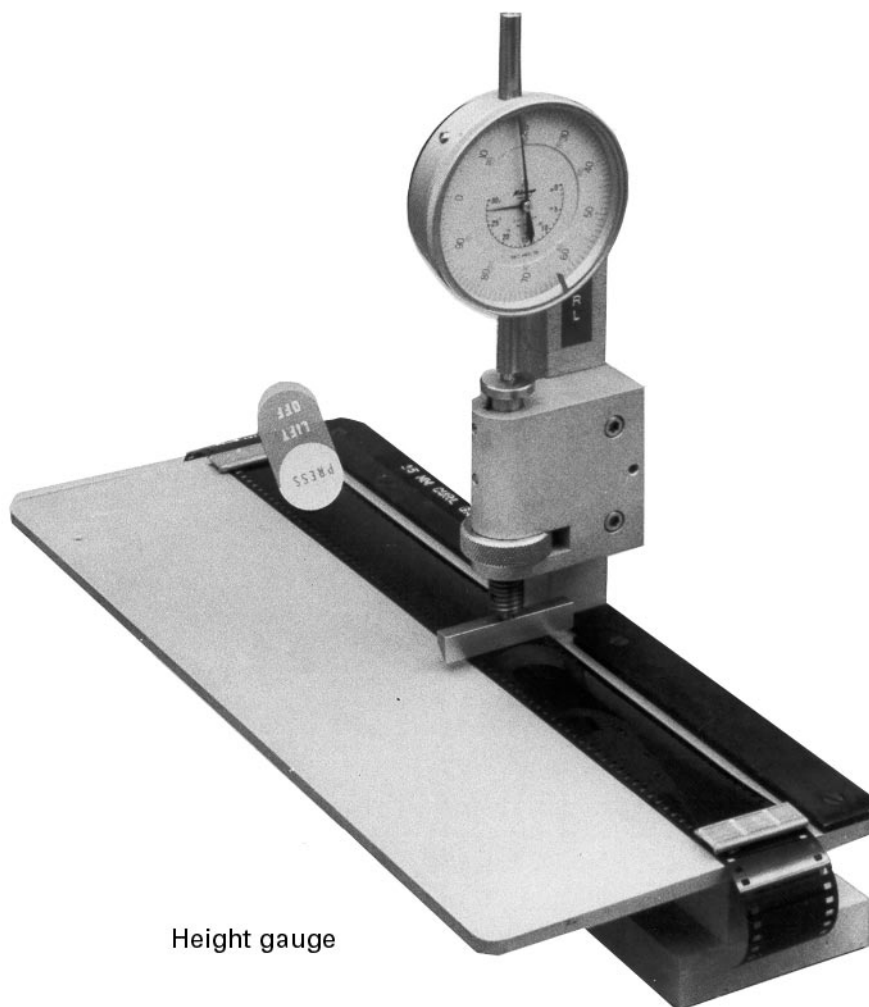
Figure 3 — Devices for reading edge curl of film strips for test method B
