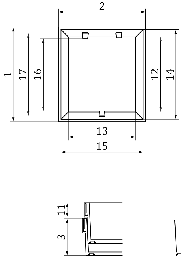
Figure 7 — Nestable and stackable boxes
