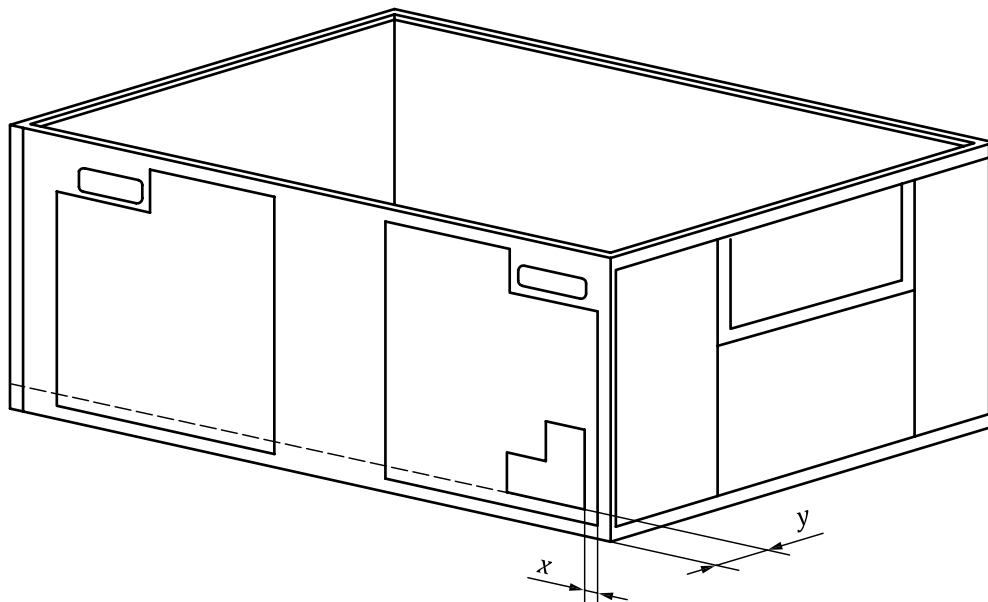
Figure 9 — Example of labelling for parallelepipedic type of box
