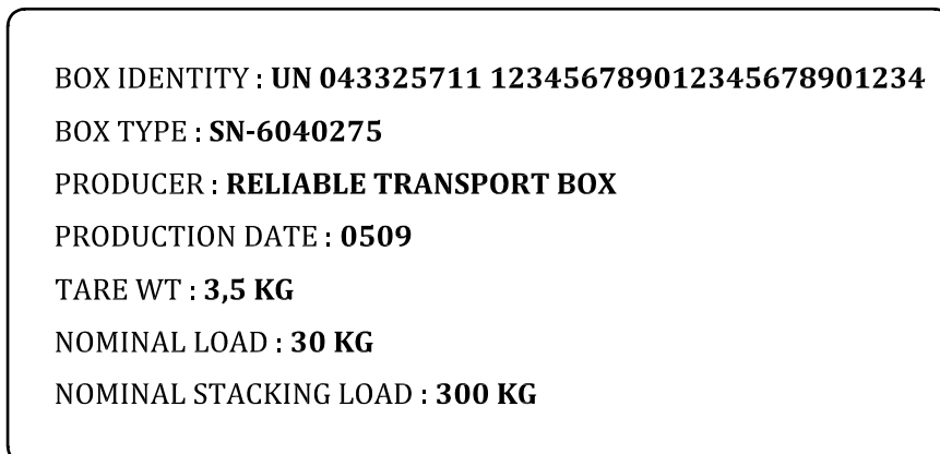
Figure 8 — Box nameplate
