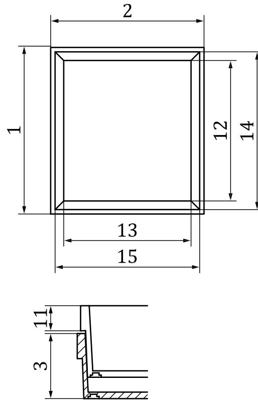
Figure 6 — Nestable box
