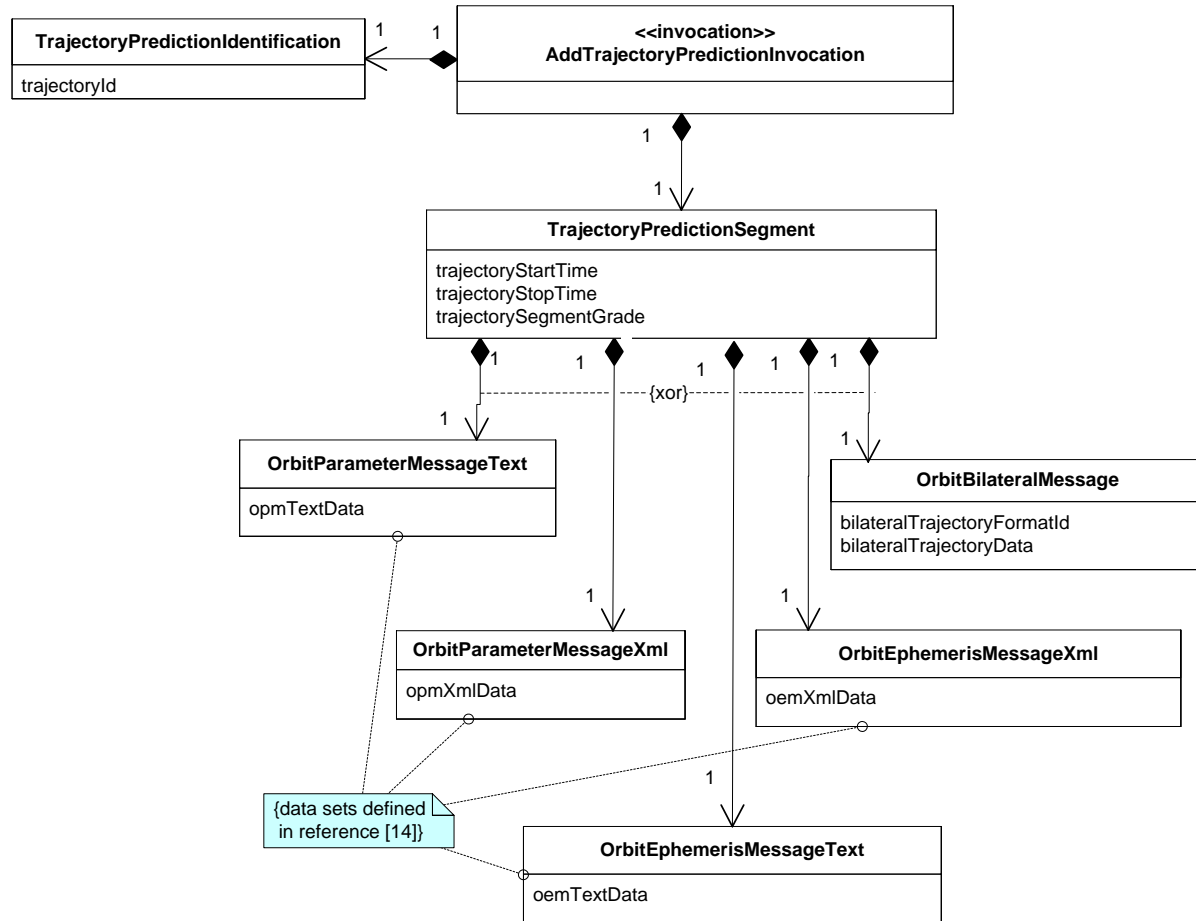
Figure 6-2: ATP-I Message Structure Class Diagram
