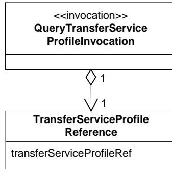
Figure 5-37: QTSP-I Message Structure Class Diagram
