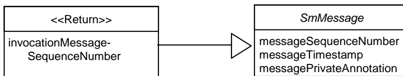
Figure 3-10: <<Return>> Message Stereotype Class Diagram
