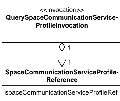
Figure 5-10: QSCSP-I Message Structure Class Diagram
