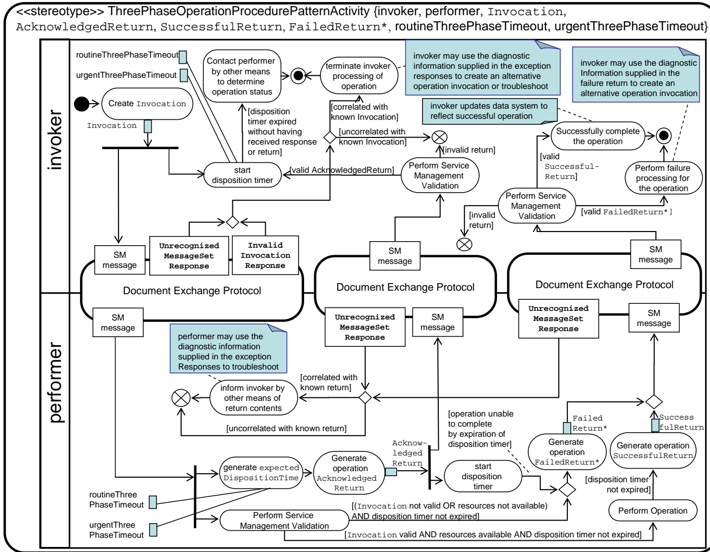
Figure 3-25: Three-Phase Operation Procedure Pattern Activity Diagram
