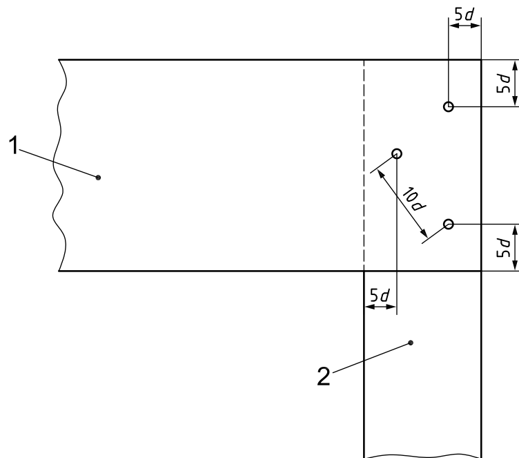
a) Example of nail spacing for block-type pallets
