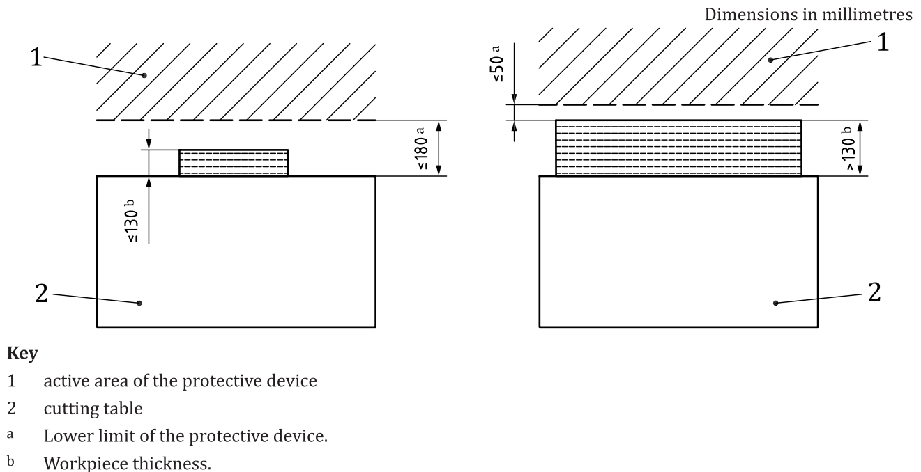
Figure C.1 — Lower limit of the protective device
