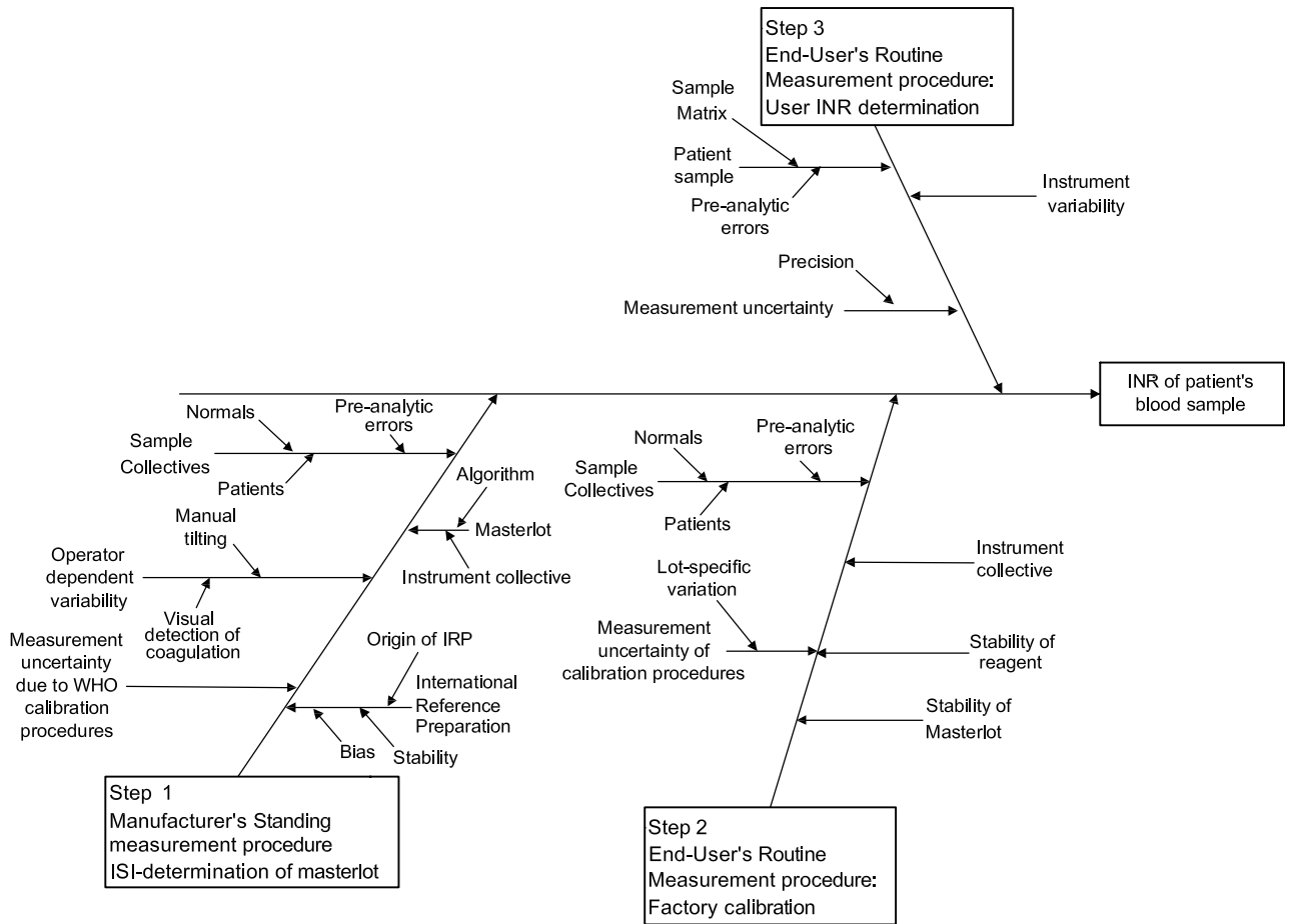
Figure D.1 — Cause and effect diagram of the traceability chain of a prothrombin INR determination of an anticoagulated patient
