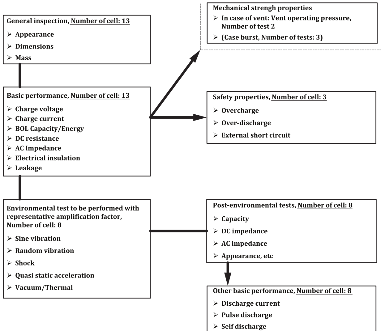
Figure B.1 — Cell qualification test flow
