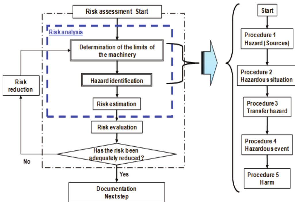
Figure C.1 — Hazard identification method
