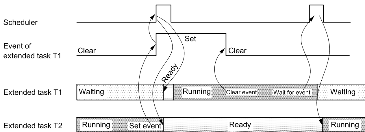
Figure 10 — Synchronization of preemptible extended tasks
