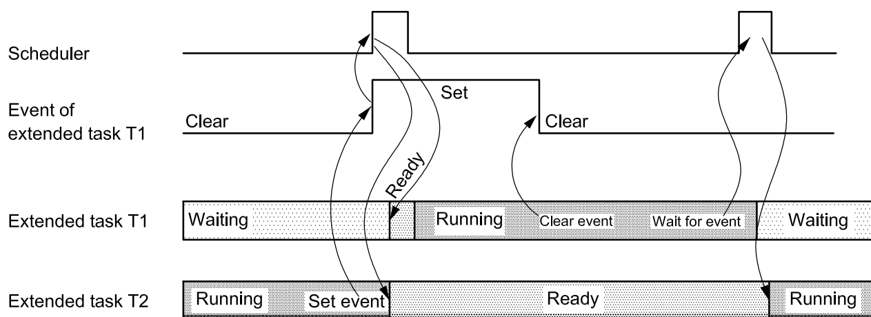
Figure 11 — Synchronization of non-preemptible extended tasks
