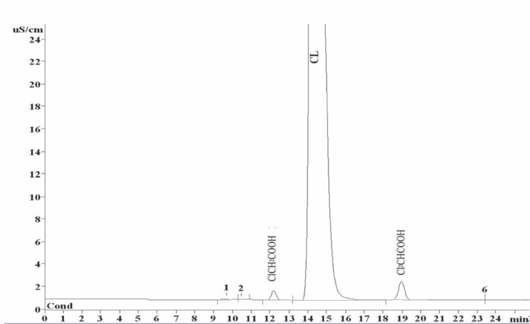
Figure A.1 — A typical IC chromatogram for monochloroacetic acid and dichloroacetic acid (on IC condition 1)
