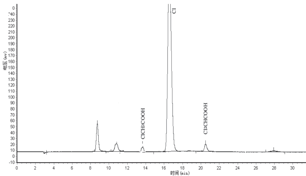
Figure A.2 — A typical IC chromatogram for monochloroacetic acid and dichloroacetic acid (on IC condition 2)
