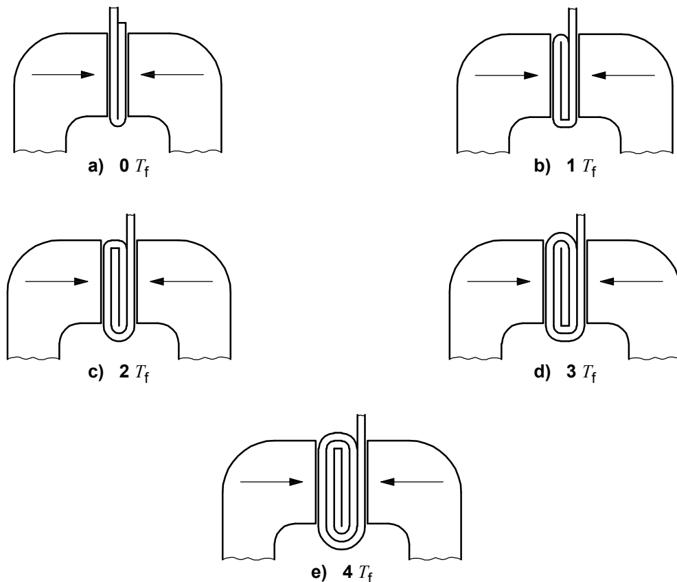
Figure 3 — Folding method
