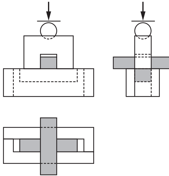
b) Ball-shaped pressure head
