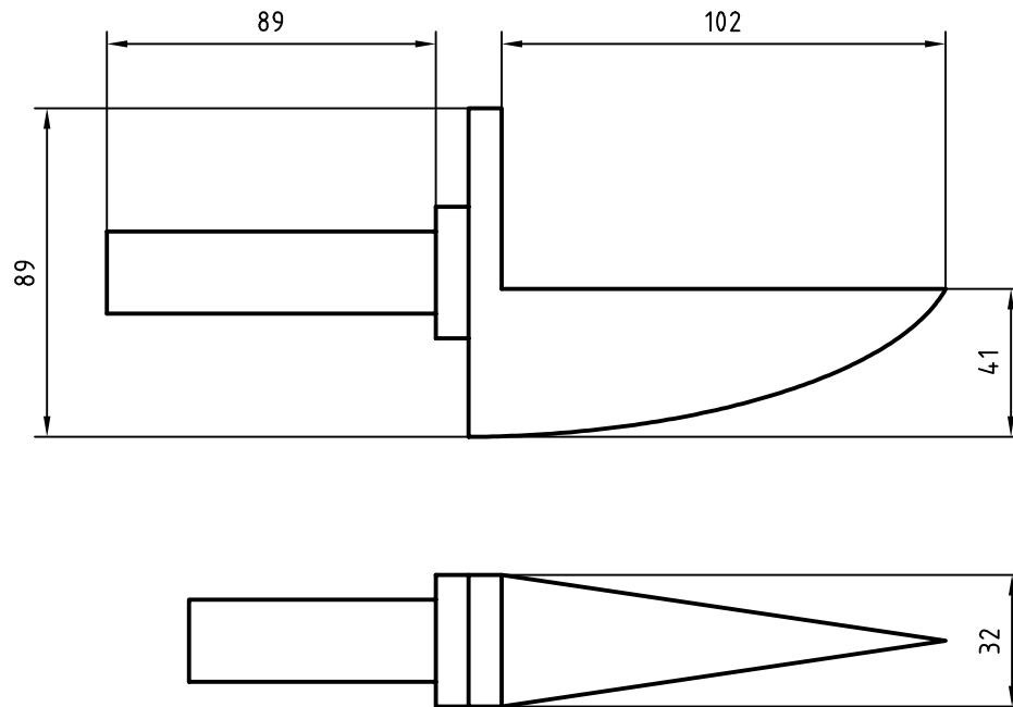
Figure A.3 — Sharp impactor
