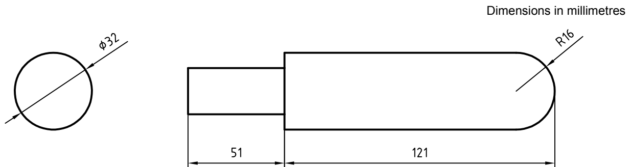
Figure A.2 — Small blunt impactor
