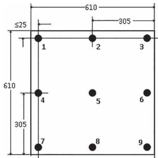
Figure 10 — Downstream mixing aerosol injection grid
